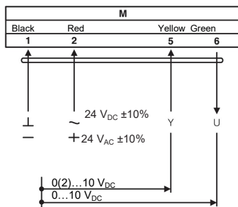
Wiring diagram NECM...05 (S1) Power supply 24 V AC / DC
