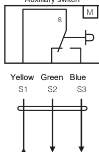
Wiring diagram MECA...05 (S1) Auxiliary switch
