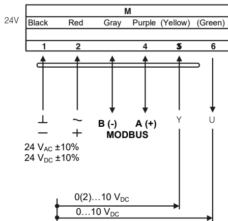
Wiring diagram MECA...05 (S1) Power supply 24 V AC / DC
